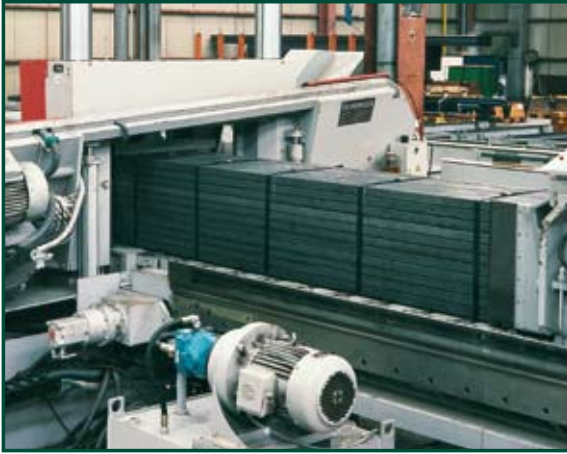
Sawing to size.
